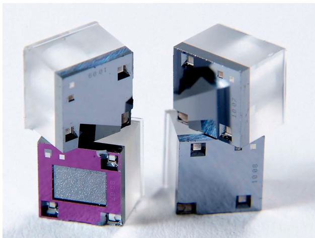
Figure 2: TERPS Sensor Element
