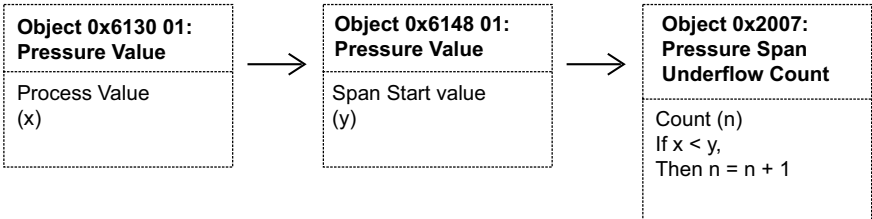
Figure 9: Pressure Span Underflow Count
