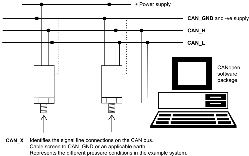
Figure 1: An Example CAN bus System
